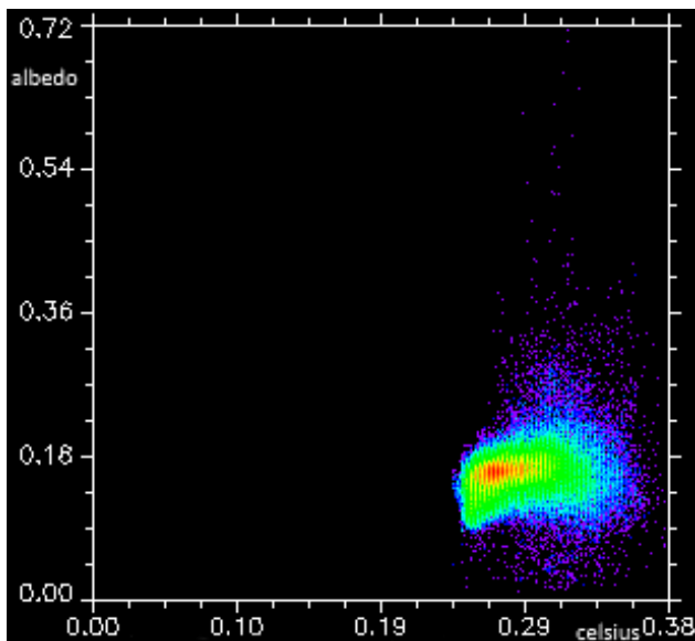
Figure 11. The 2D scatterplot between Celsius (X axis) and Albedo (Y axis).
