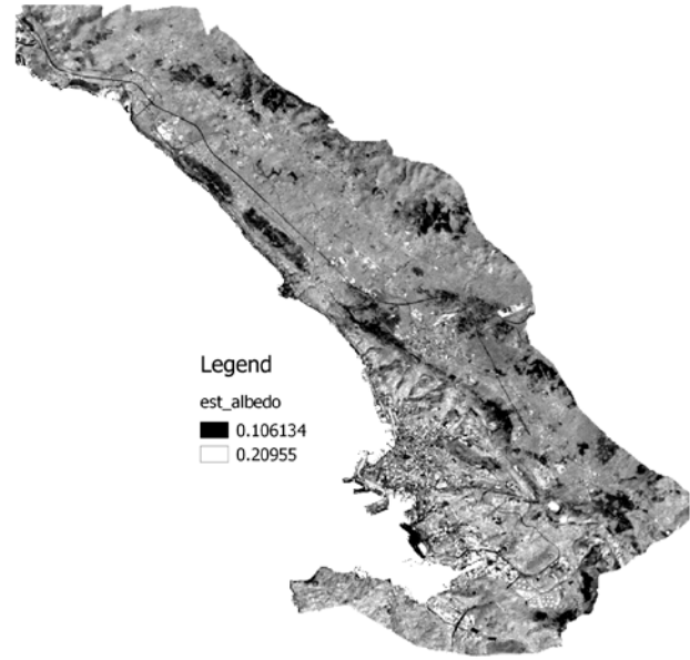
Figure 5. The albedo map of Landsat 8 image (Province of Trieste).
